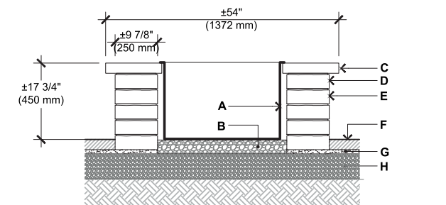
SECTION 1-1
