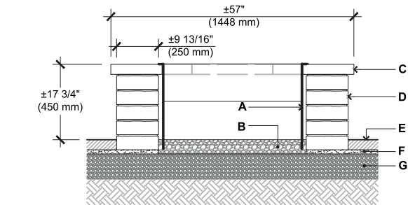
SECTION 1-1
