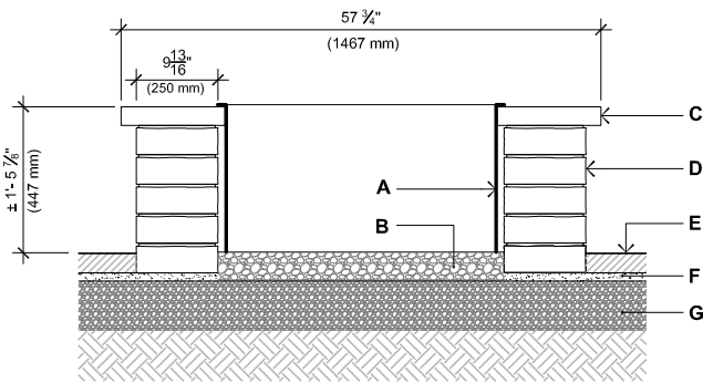
SECTION 1-1
