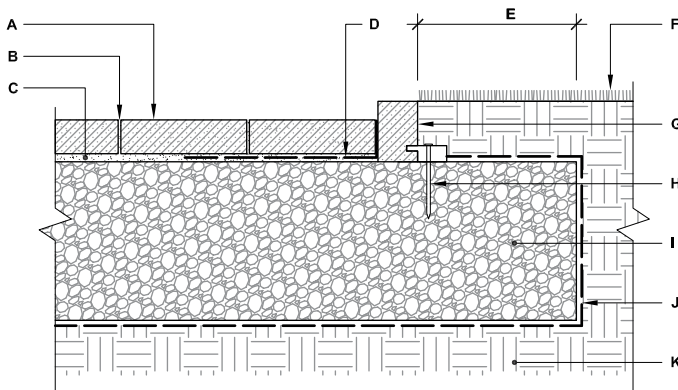
TYPICAL PAVER CROSS SECTION WITH PIETRA EDGE
