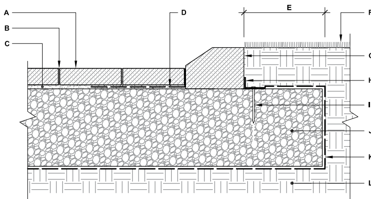
TYPICAL PAVER CROSS SECTION WITH TUNDRA EDGE
